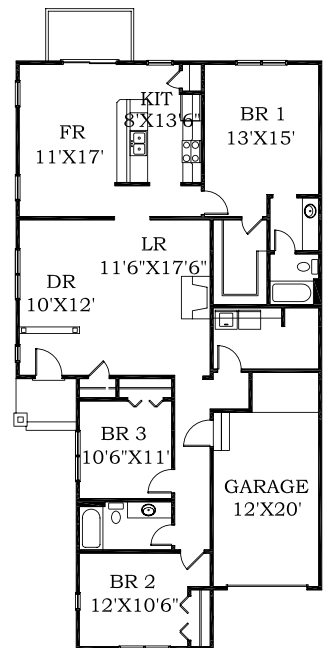
Floor Plan with Crawlpace
