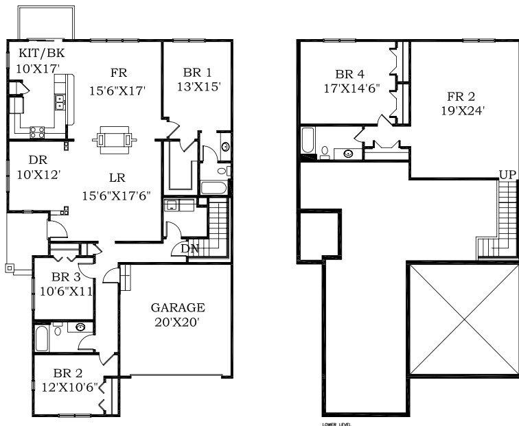
Floor Plan with Basement
