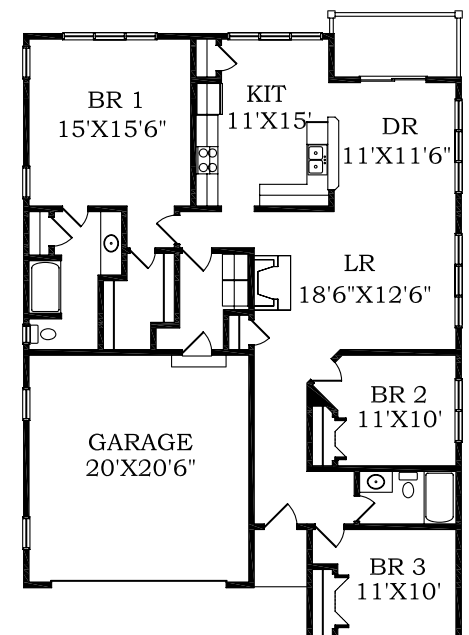
Floor Plan with Crawlpace
