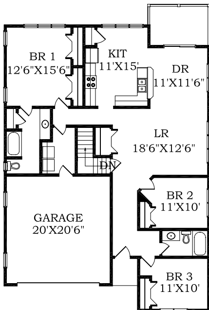
Floor Plan with Basement
