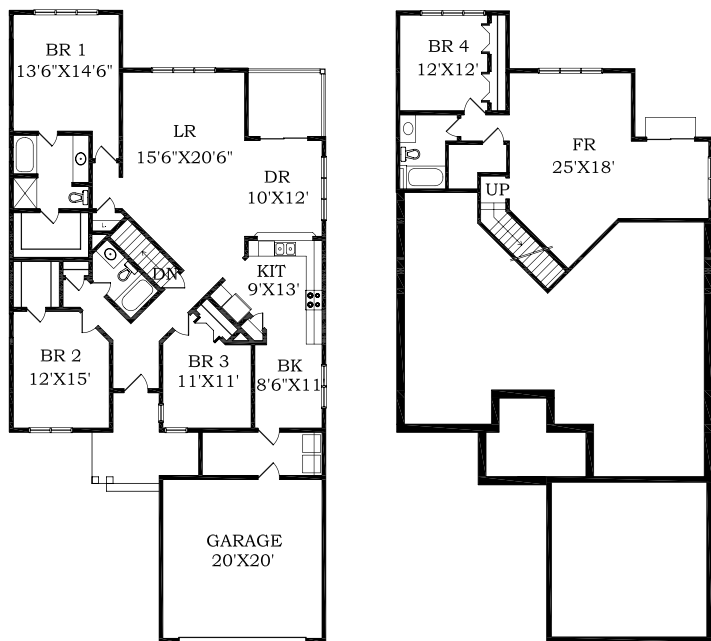
Floor Plan with Basement
