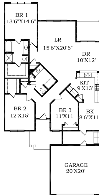
Floor Plan with Crawlspace
