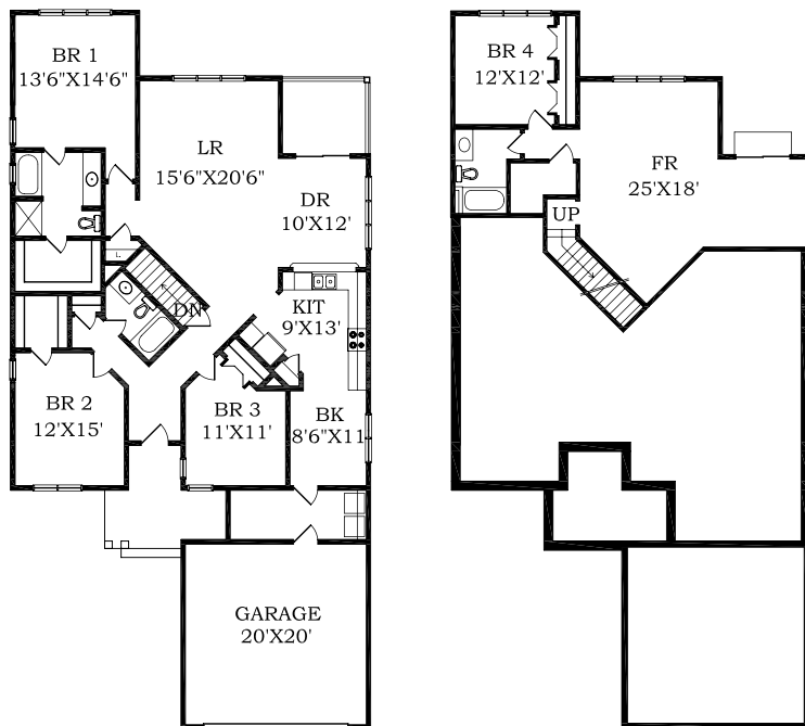
Floor Plan with Basement
