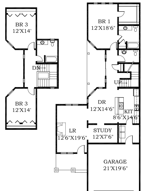
Floor Plan with Crawlpace
