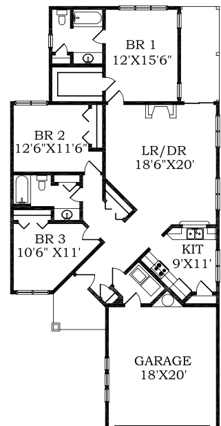
Floor Plan with Crawlspace
