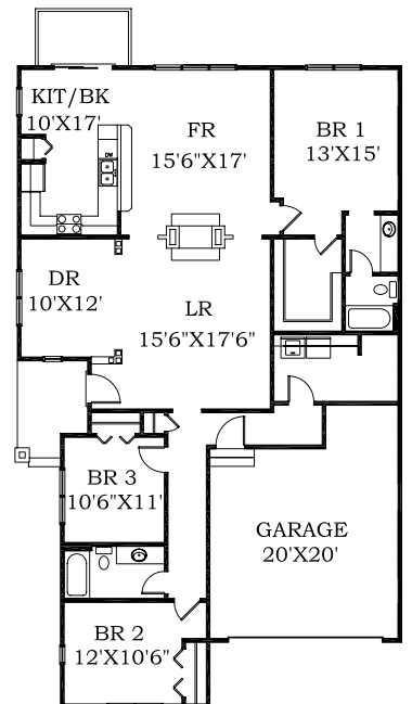
Floor Plan with Crawlspace
