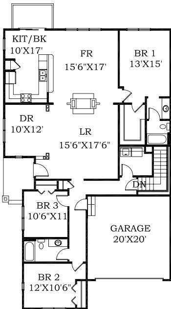
Floor Plan with Basement
