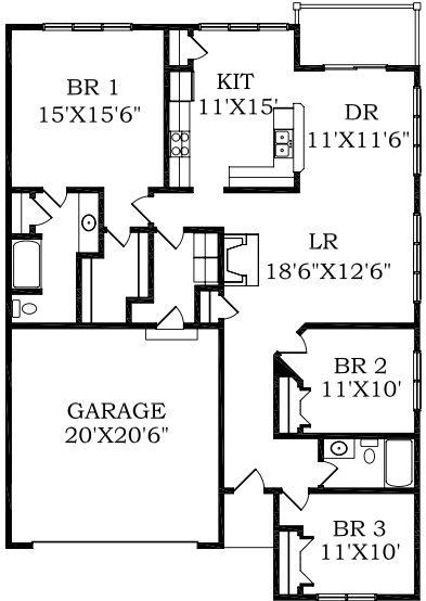
Floor Plan with Crawlspace
