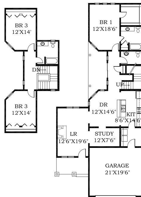
Floor Plan with Crawlspace
