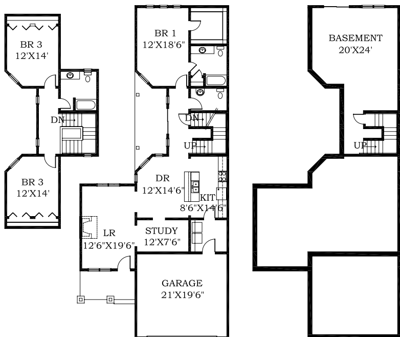
Floor Plan with Basement
